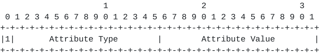
Figure 6: Data Attributes
