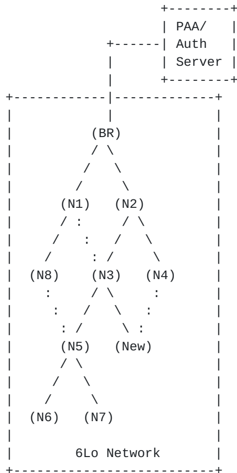
Figure 1: Sample Topology
