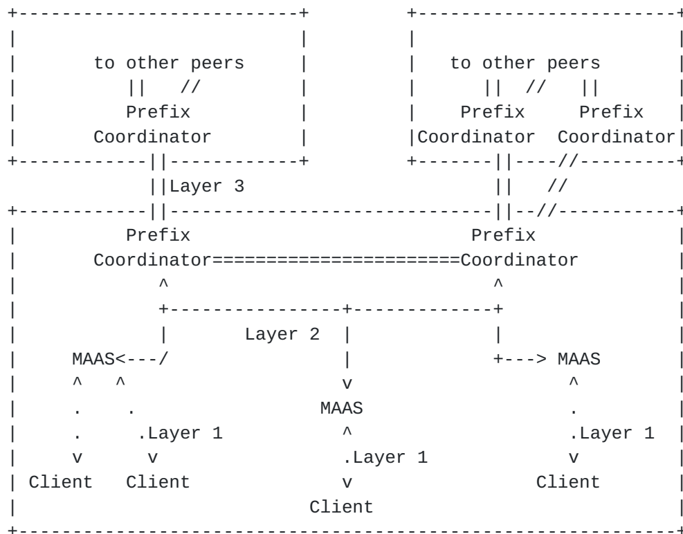
Figure 1: An Overview of the Multicast Address Allocation Architecture
