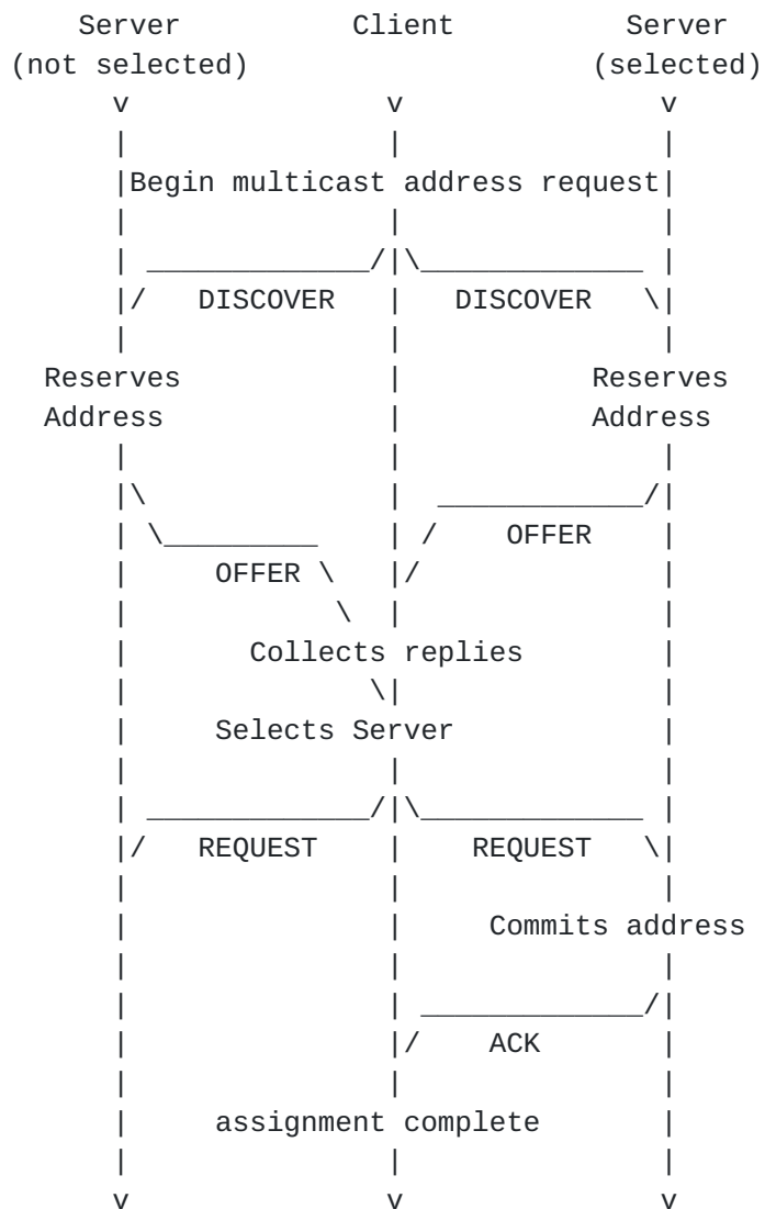
Figure 3: Timeline diagram of messages exchanged in Multicast Address Allocation example
