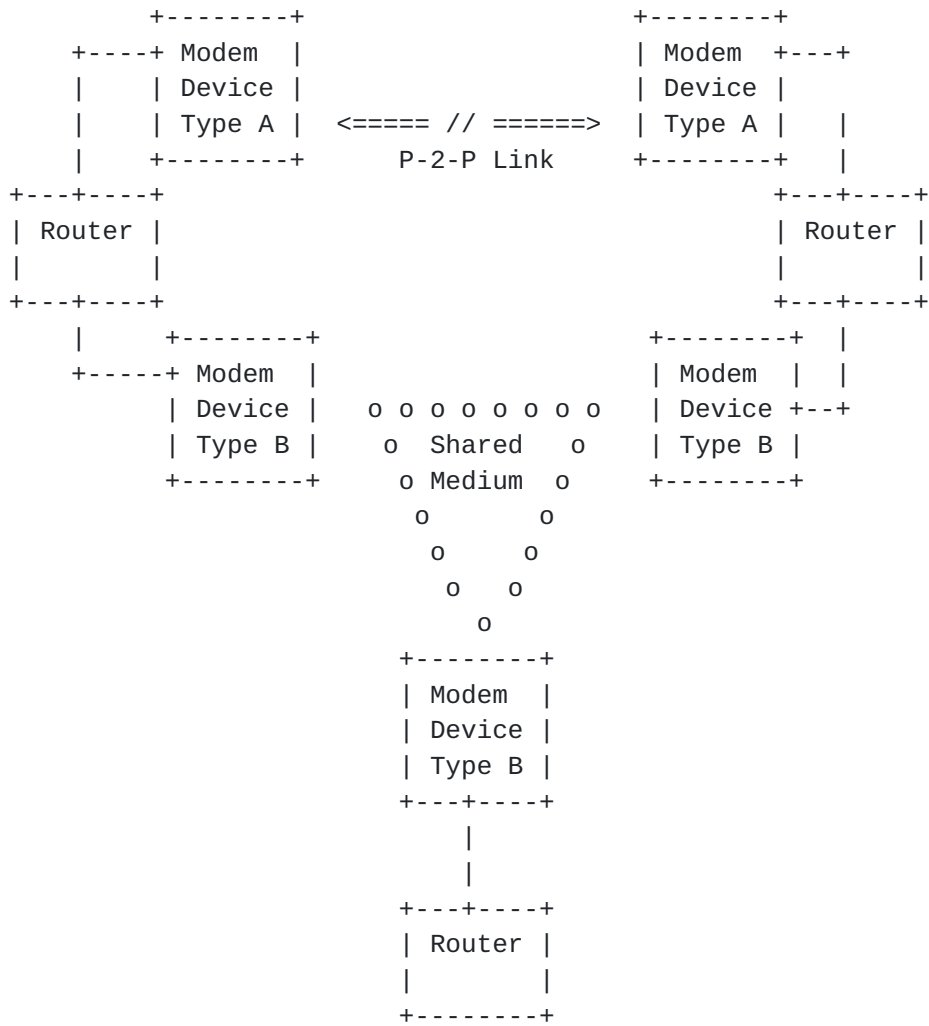
Figure 2: DLEP Network with Multiple Modem Devices
