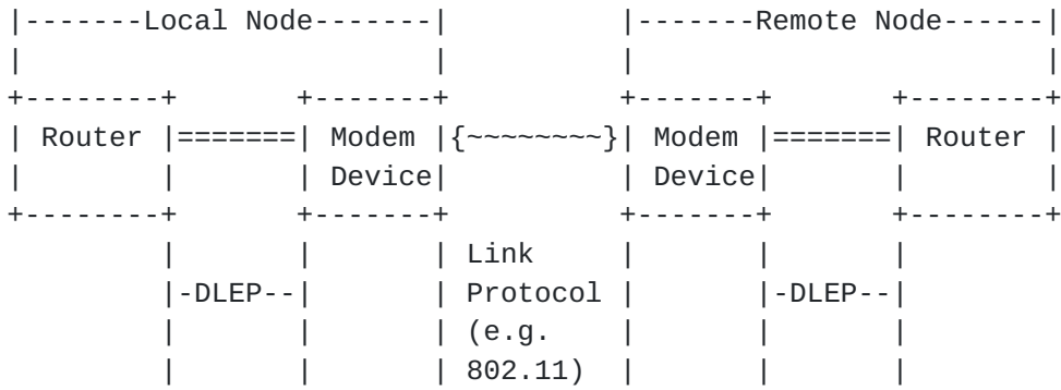
Figure 1: DLEP Network
