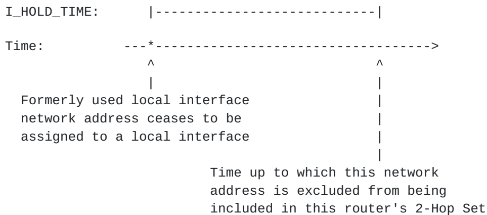
Figure 11: Local interface removed network address
