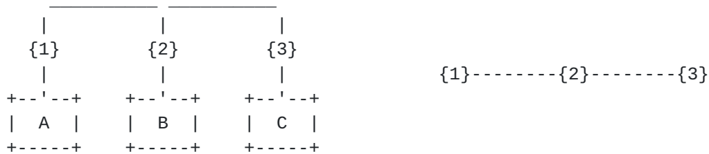
Figure 12: Standard single interface topology (left), and corresponding NHDP representation (right)
