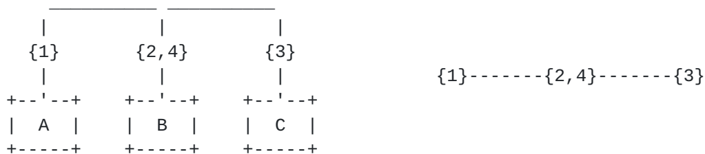
Figure 13: Single interfaces, with 1-hop neighbor B having two addresses (left), and corresponding NHDP representation (right)
