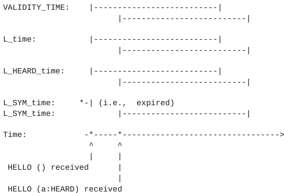
Figure 7: HELLO message processing: network address present
