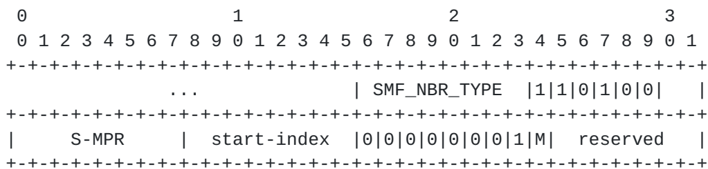
Figure 9: S-MPR Address Block TLV Example
