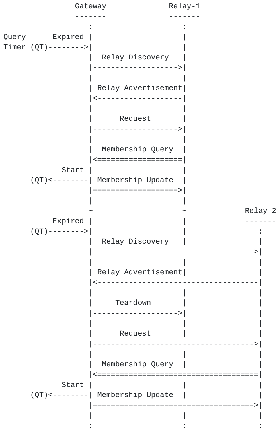
Teardown After Relay Address Change
