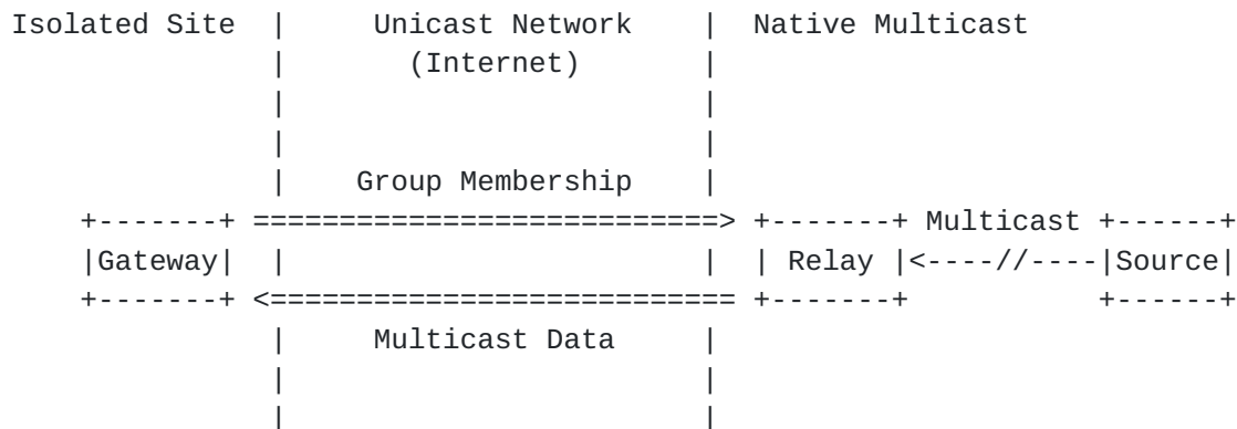
Figure 1: Basic AMT Architecture
