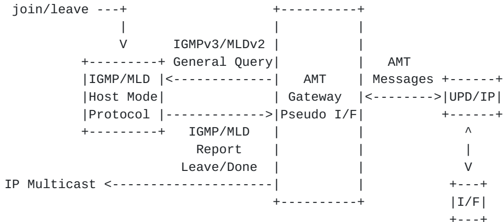
Figure 2: AMT Gateway Pseudo-Interface
