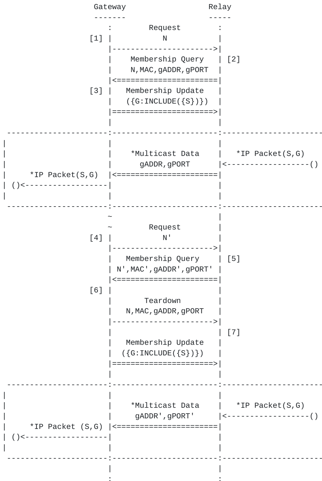
Figure 3: Teardown Message Sequence (IGMPv3/MLDv2 Example)
