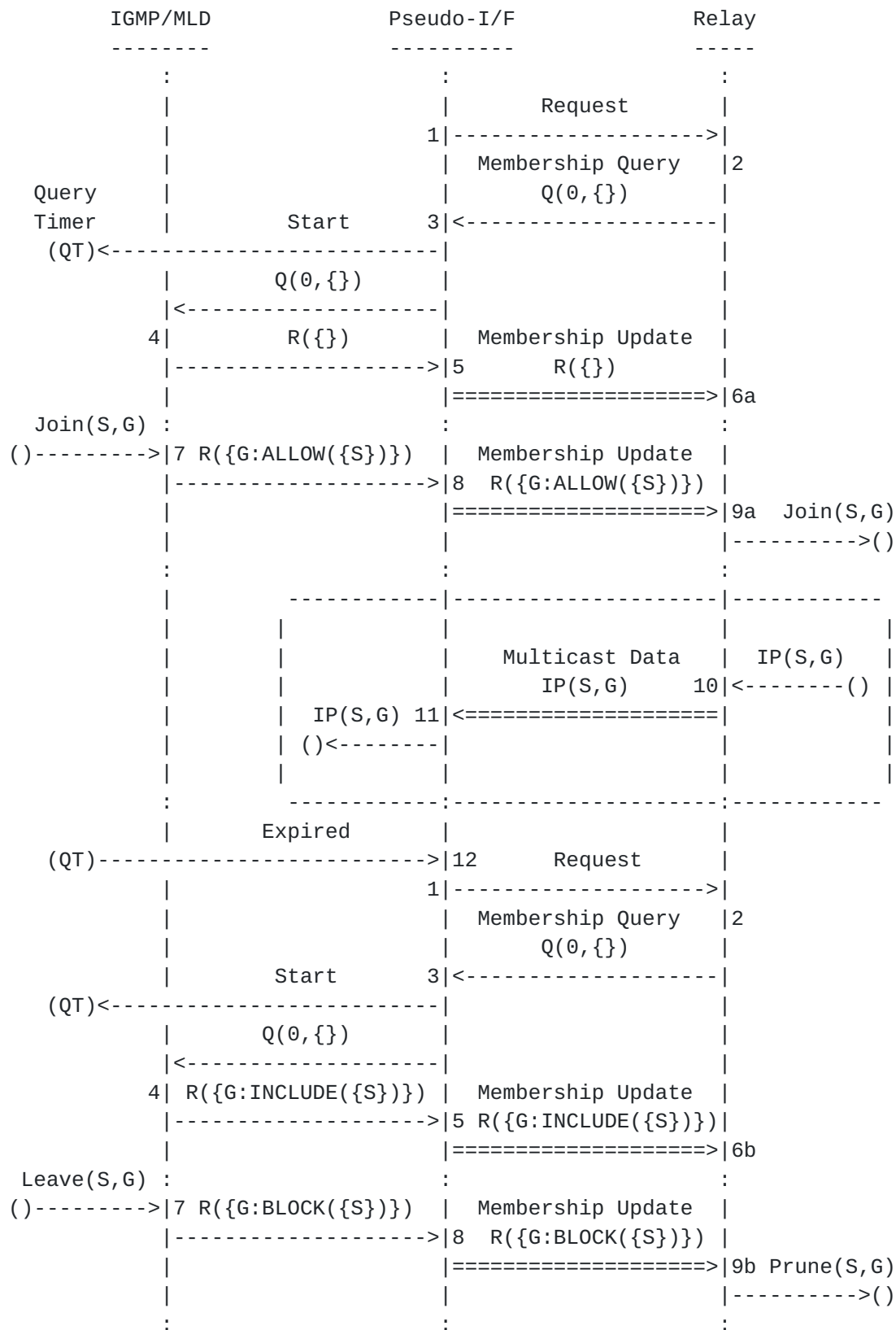
Membership Update Sequence (IGMPv3/MLDv2 Example)
