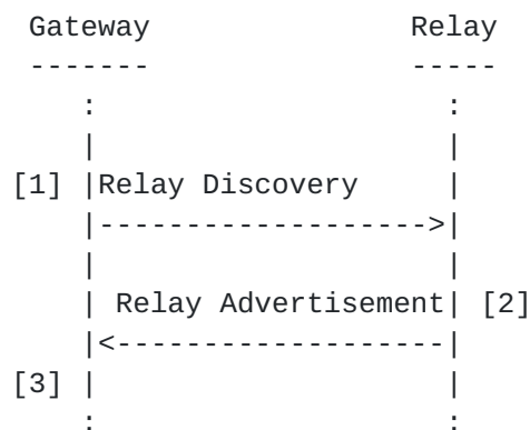
AMT Relay Discovery Sequence
