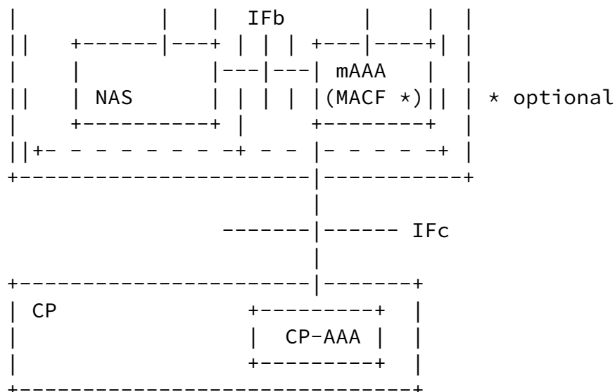
Figure 4: Fully enabled framework
