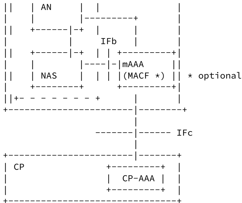
Figure 3: AAA enabled framework (basic model)
