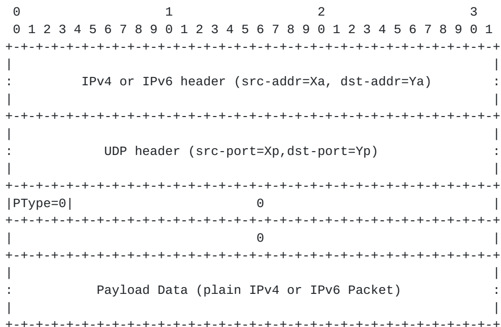
Figure 9: UDP Encapsulated Non-Protected User Data Packet Format
