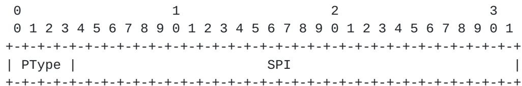
Figure 6: Security Parameter Index with Packet Type
