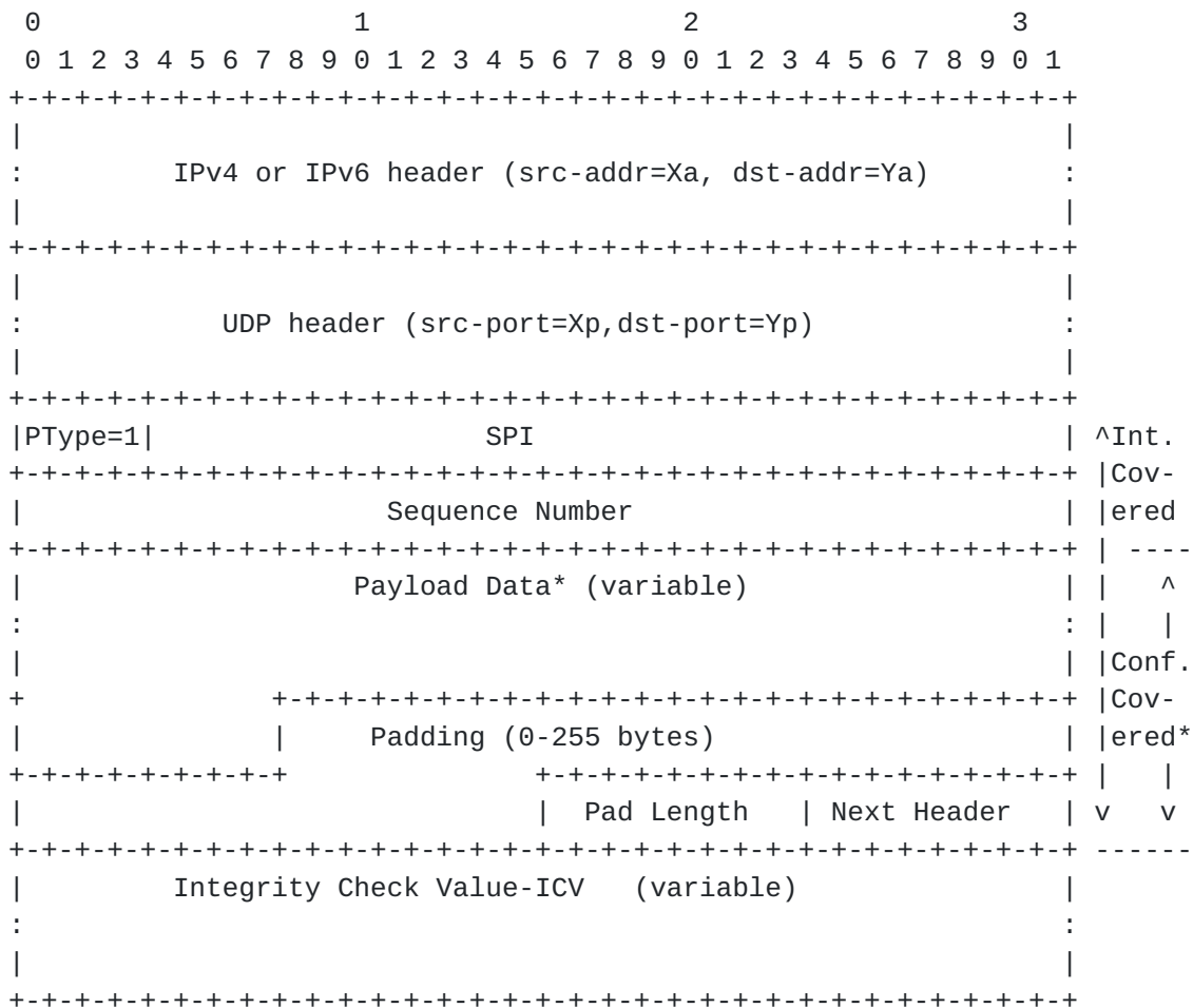
Figure 8: UDP Encapsulated Protected User Data Packet Format
