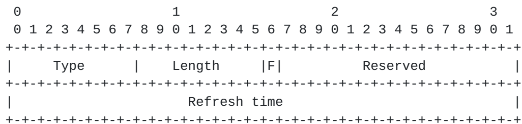
Figure 5: The NAT Detection Option
