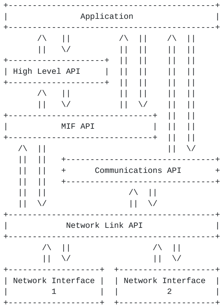
Figure 1: MIF API Elements
