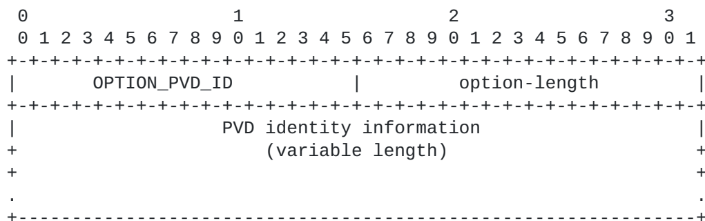
Figure 2: PVD ID Option
