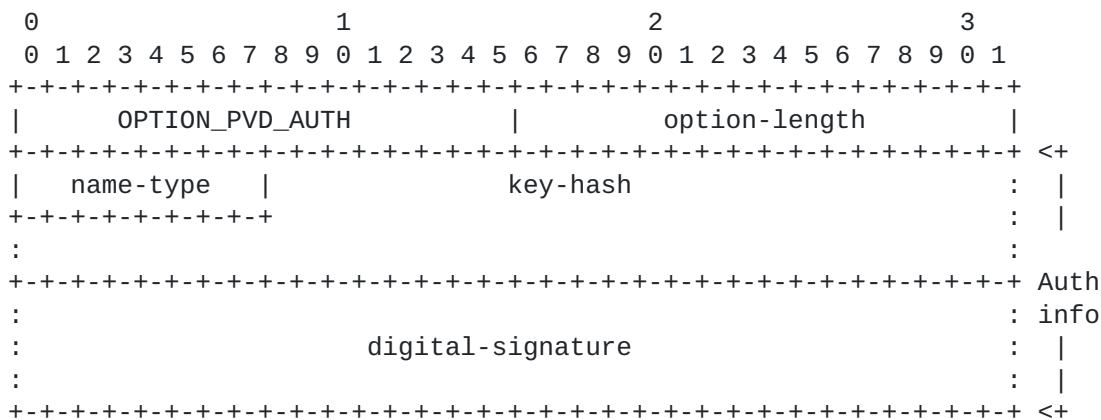
Figure 3: PVD Auth Option
