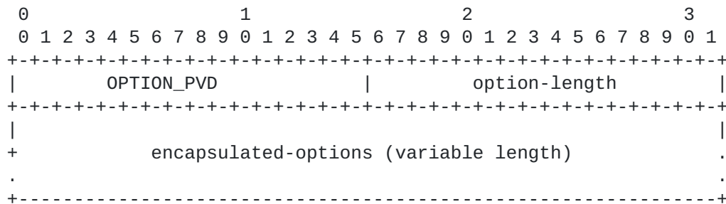
Figure 1: PVD Container Option
