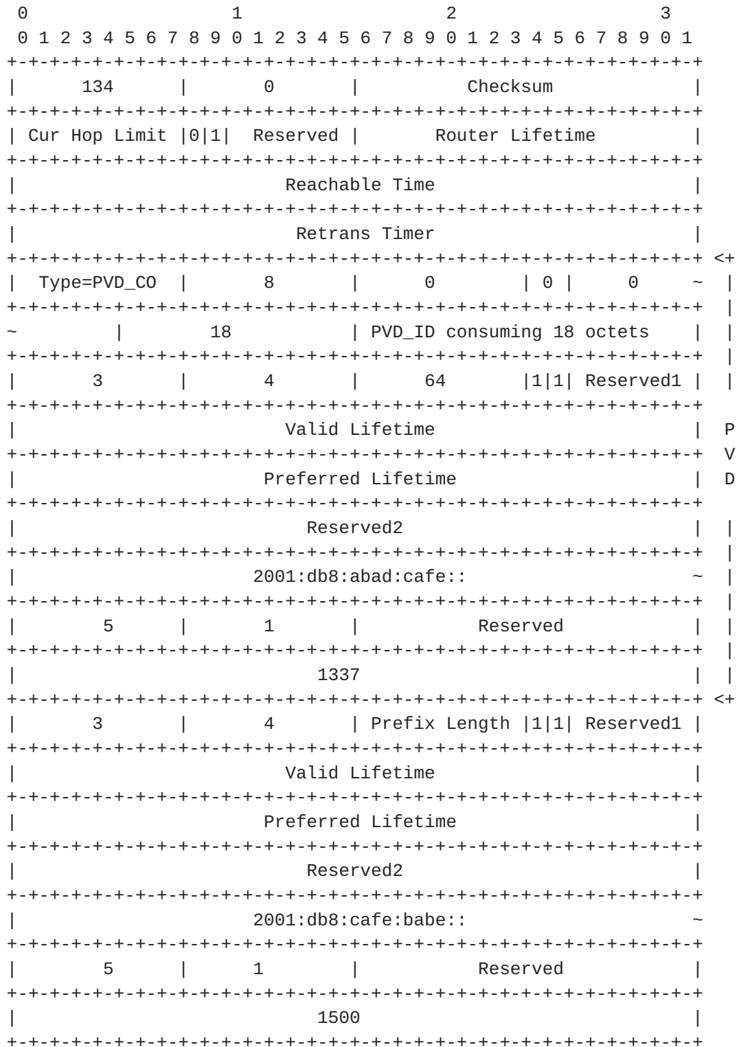
Figure 2: An RA with one implicit PVD and one explicit PVD
