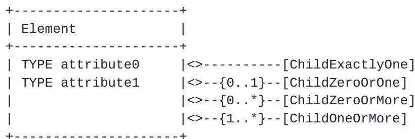
Figure 1: Example UML Element Diagram
