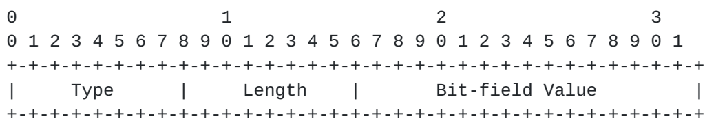
Figure 1: Multicast-Broadcast Encapsulating Extension
