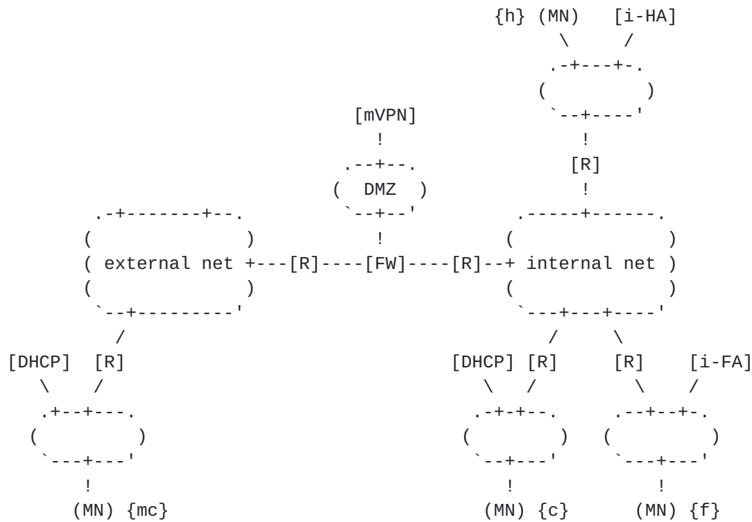
Figure 1: Network Topology using MIPv4 and MOBIKE
