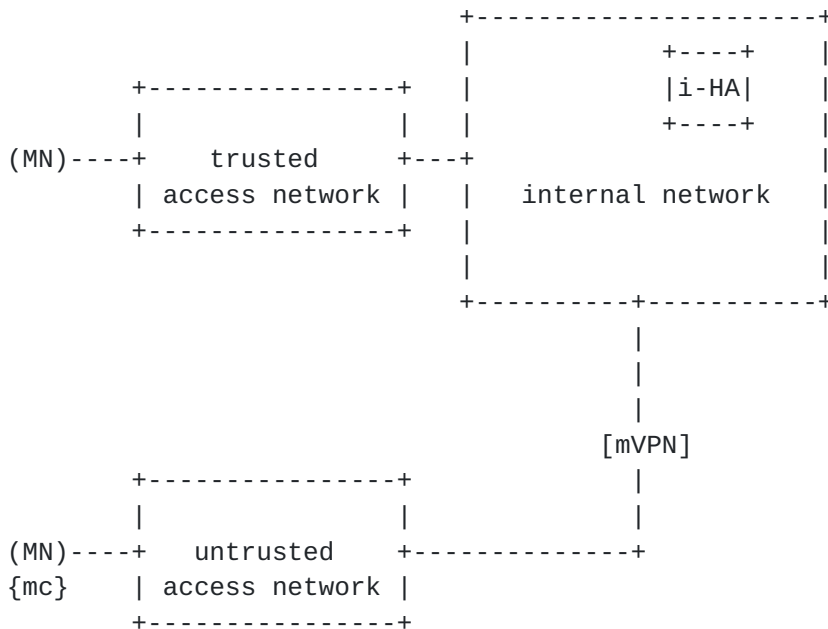
Figure 2: Network Topology of a Mobile Operator with trusted and untrusted networks
