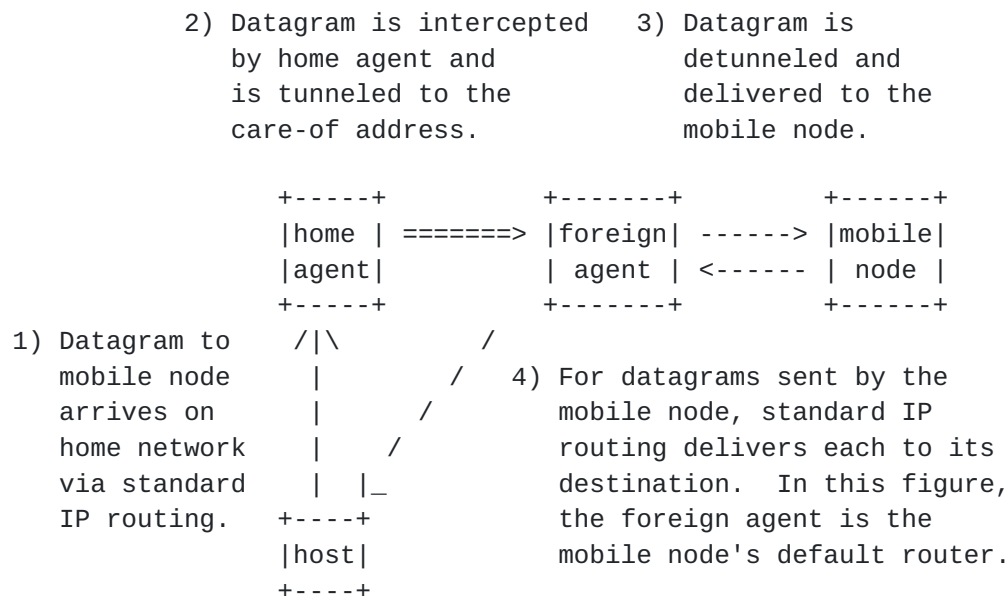
Figure 1: Operation of Mobile IPv4
