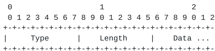
Figure 2: Type-Length-Value extension format for Mobile IPv4
