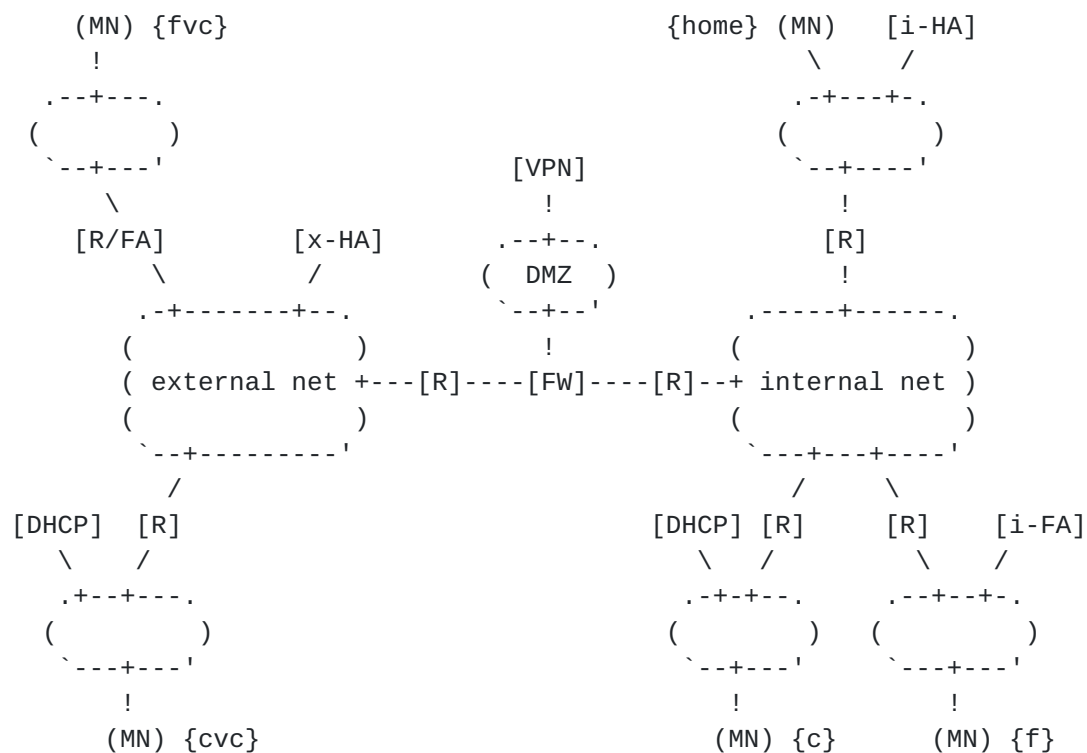
Figure: Basic topology, possible MN locations and access modes
