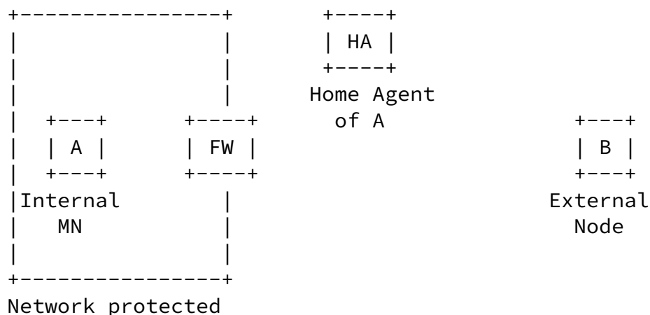
Figure 1: Issues between MIPv6 and firewalls when MN is in a network protected by firewalls
