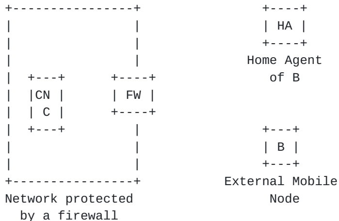
Figure 2: Issues between MIP6 and firewalls when a CN is in a network protected by firewalls
