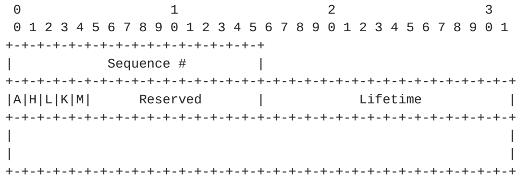
Figure 2: Local Binding Update
