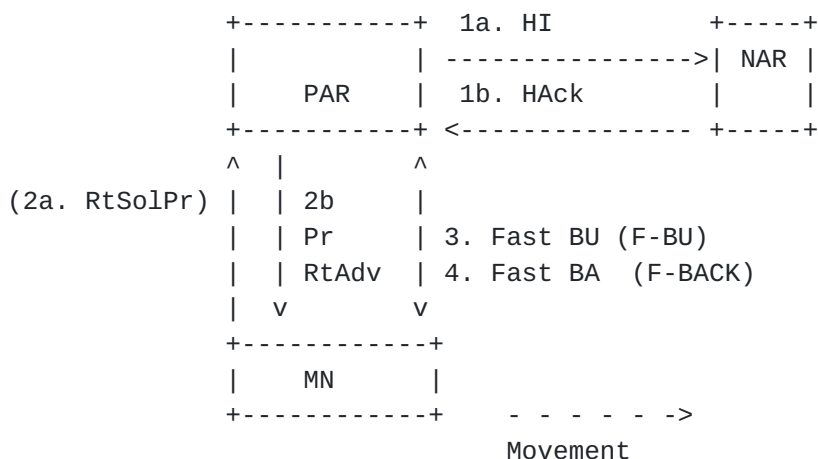
Figure A.1 - Fast Mobile IPv6 Handover Protocol
