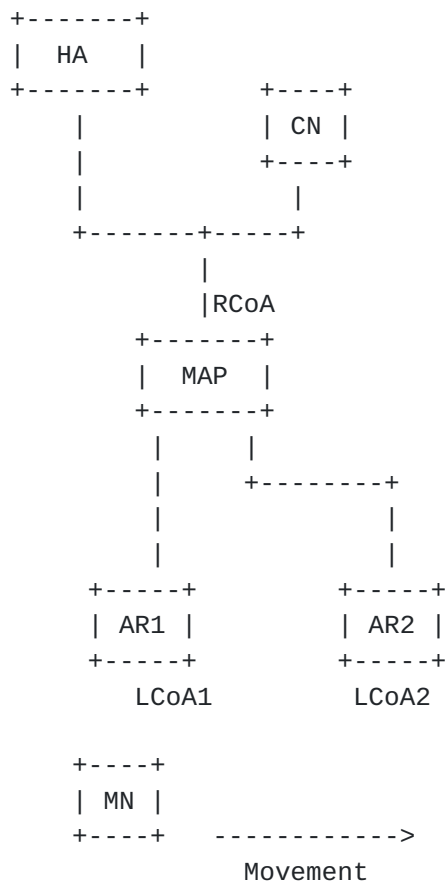
Figure 1: Hierarchical Mobile IPv6 domain
