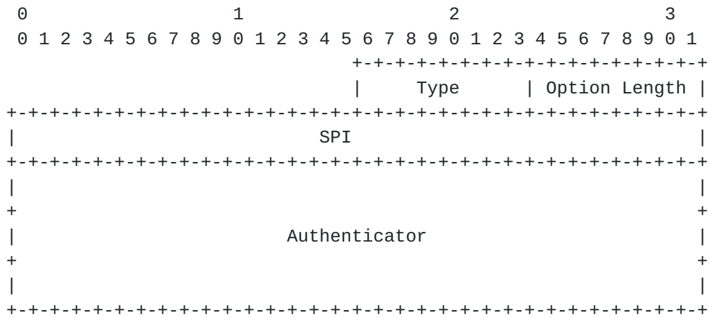
Figure 15: Binding Authorization Data for FMIPv6 (BADF) Option
