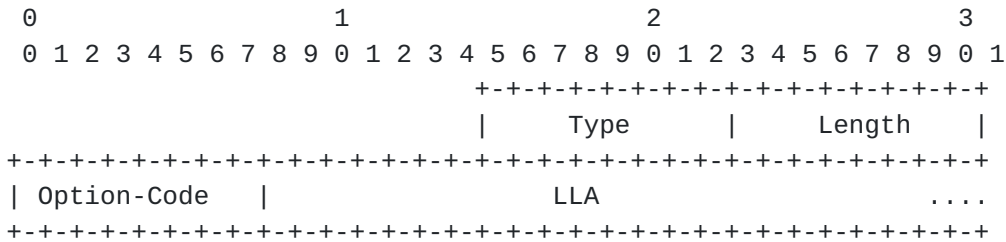
Figure 14: Mobility Header Link-Layer Address Option
