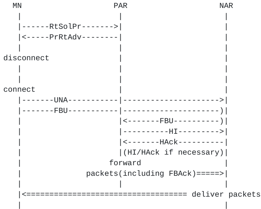
Figure 3: Reactive Fast Handover
