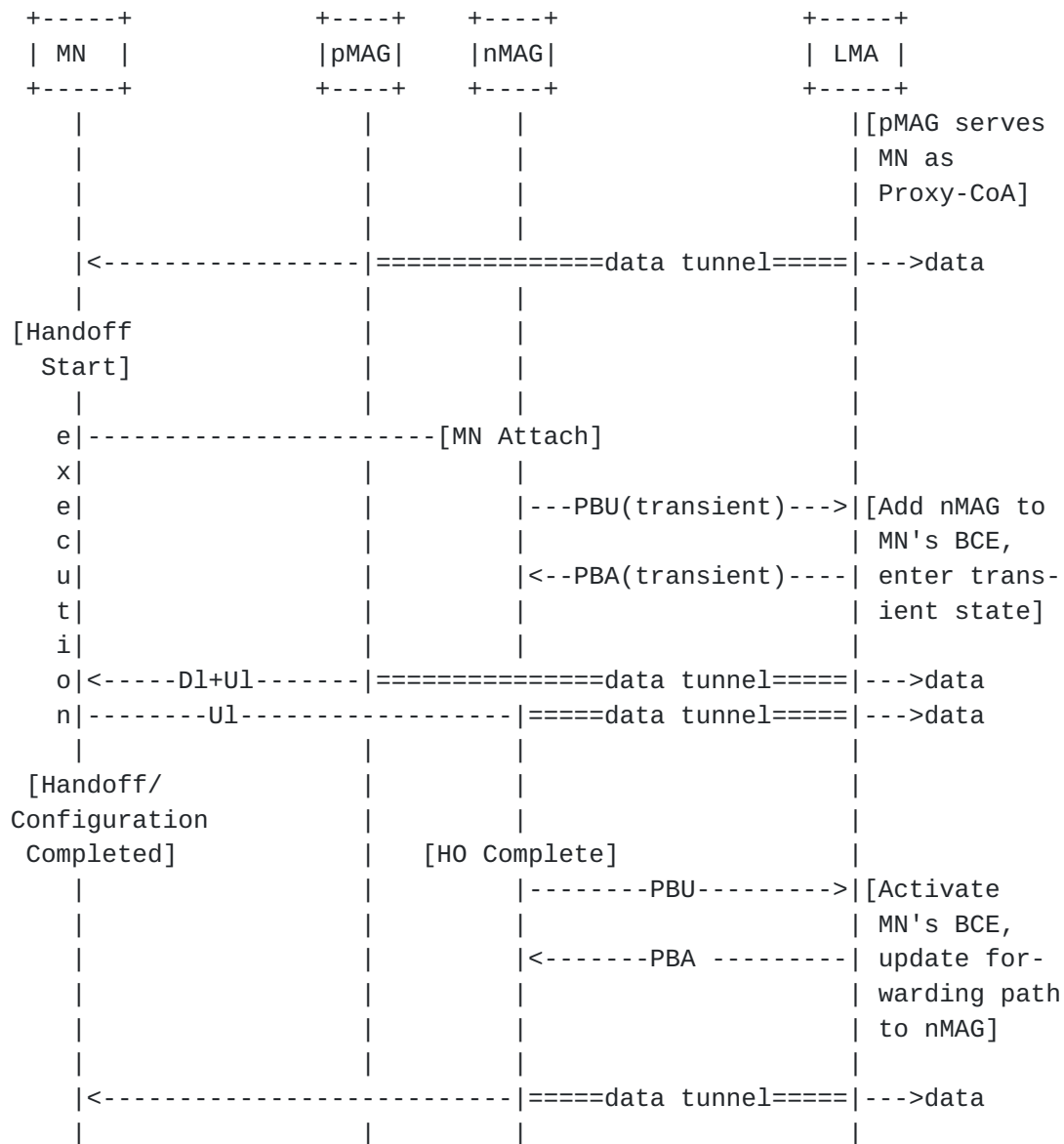
Figure 3: General mechanism and forwarding characteristics during handover with transient BCE.
