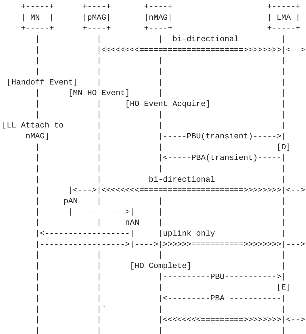
Figure 5: Transient BCE support for an intra-technology handover
