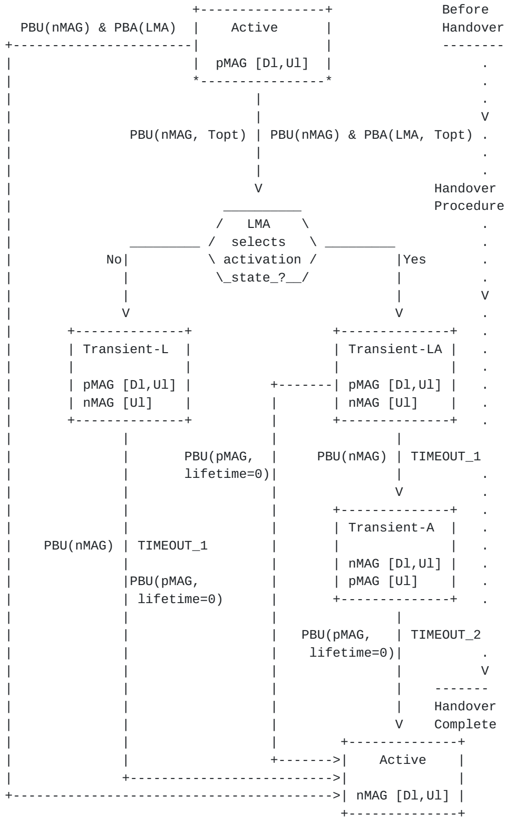
Figure 4: Possible transient forwarding states during a handover.
