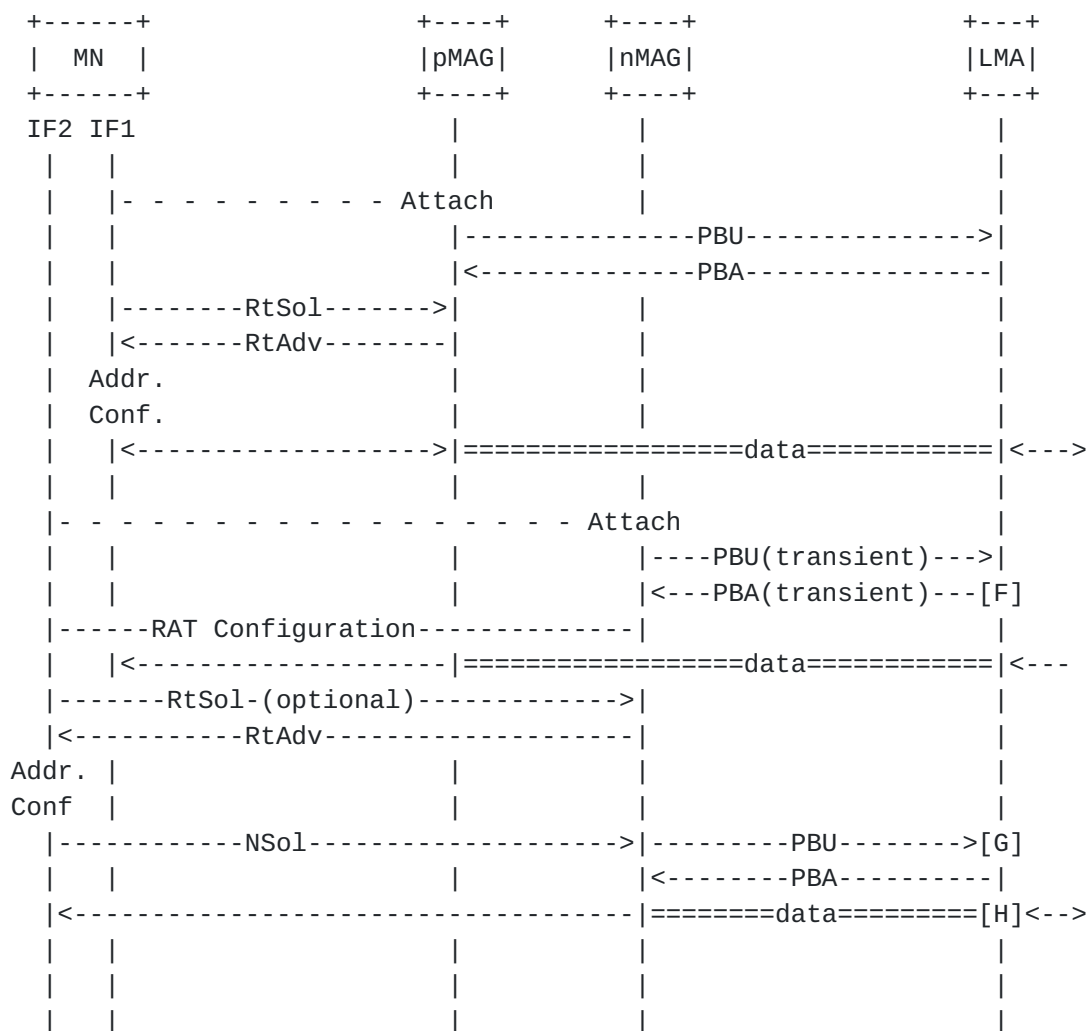
Figure 6: Late path switch with PMIPv6 transient BCEs.
