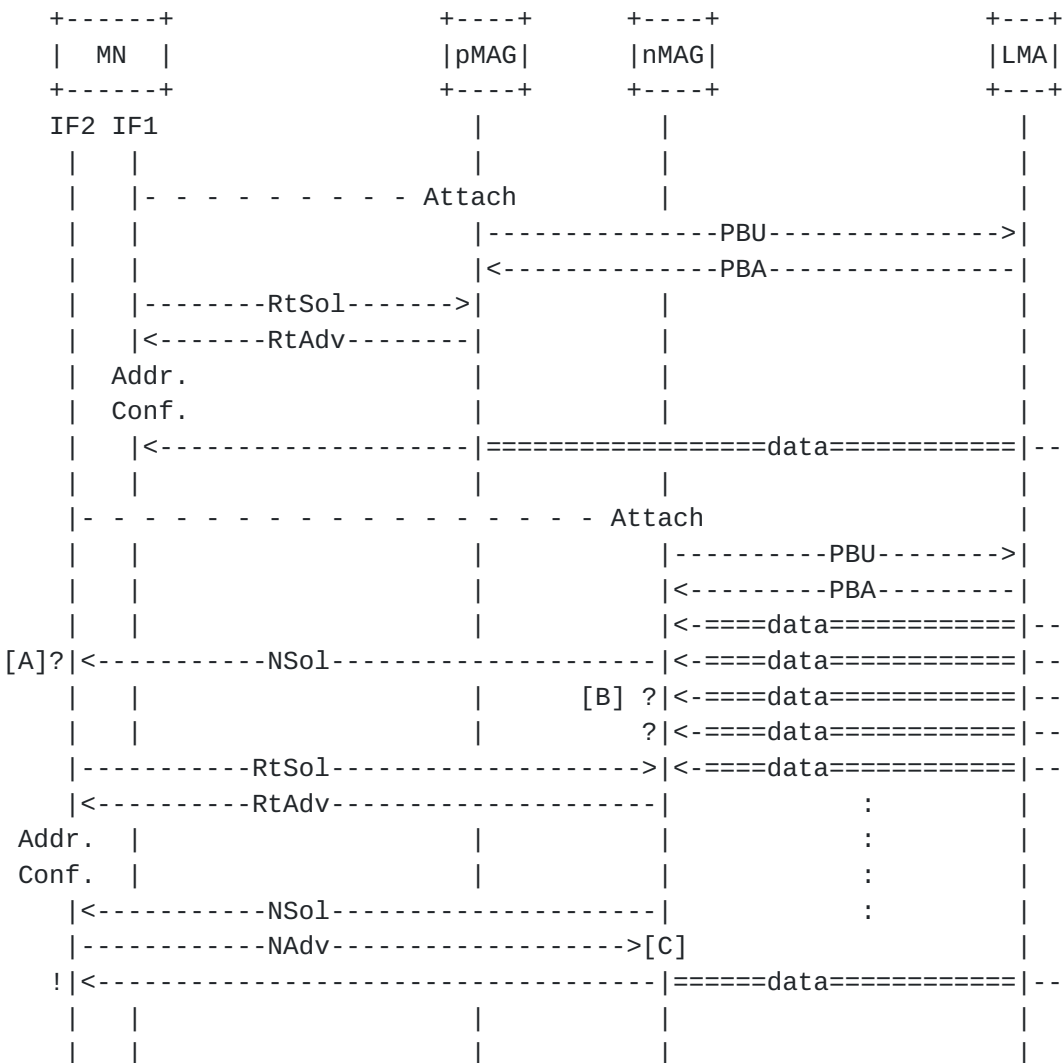
Figure 1: Issue with dual radio handover.
