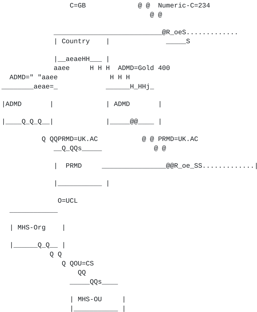
Figure 1: Example O/R Address Tree
