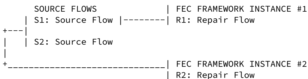
Figure 1: Example scenario with two FEC Framework instances where R1 protects S1, and R2 protects the group of S1 and S2
