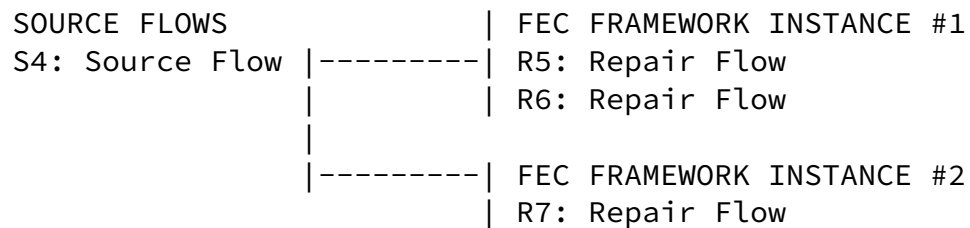
Figure 3: Example scenario with two FEC Framework instances, where two repair flows in the first instance and a single repair flow in the second instance protect the same source flow S4
