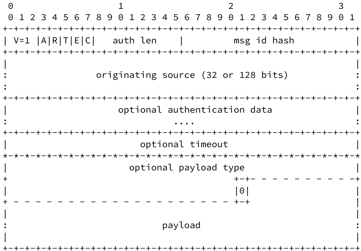
Figure 1: Packet format
