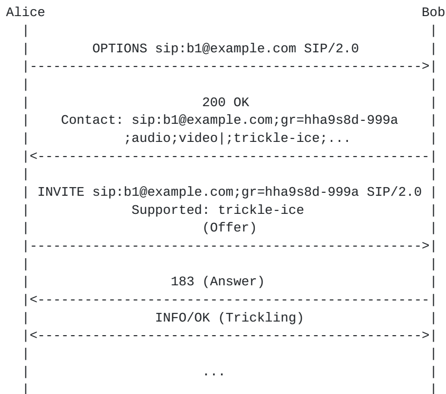
Figure 8: Trickle ICE support discovery with OPTIONS and GRUU
