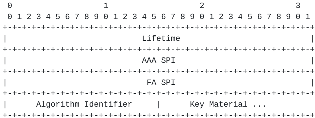
Figure 1: The Unsolicited MN-FA Key Material From AAA Subtype-Specific Data
