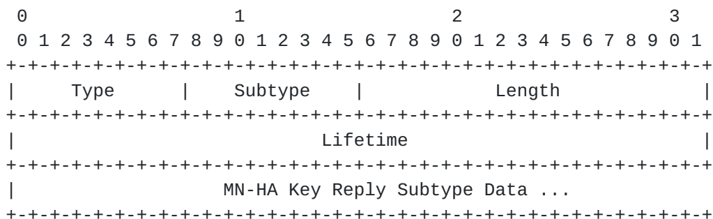
Figure 4: The Generalized Mobile IP MN-HA Key Reply Extension
