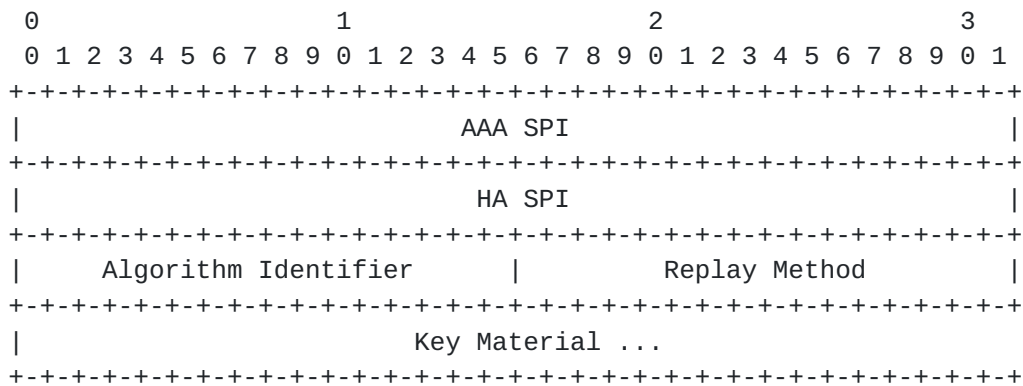
Figure 6: The MN-HA Key Material From AAA Subtype-Specific Data
