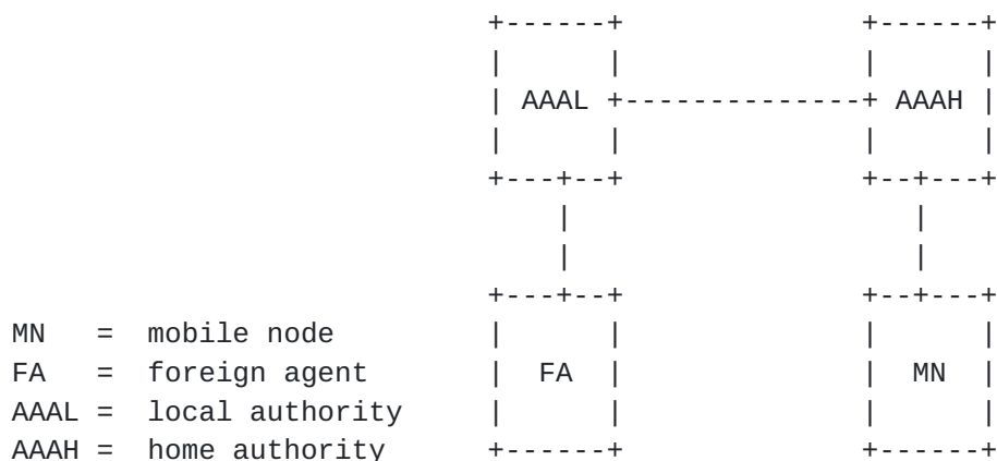
Figure 8: Security Associations
