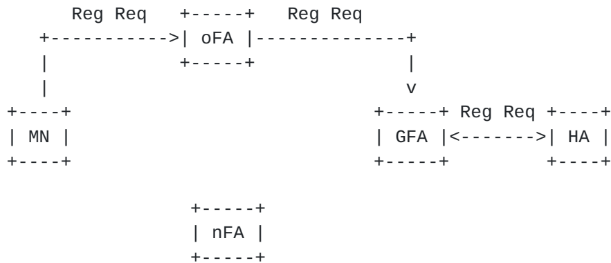
Figure A.1 - Initial Registrations through GFA
