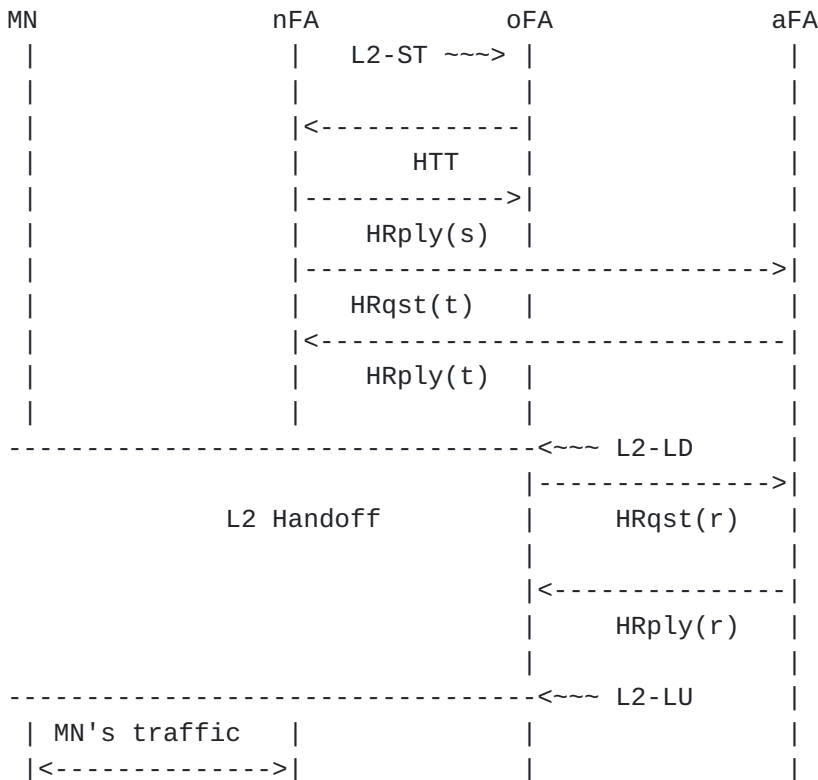
Figure 10 - Three Party Source Trigger Handoff Timing
