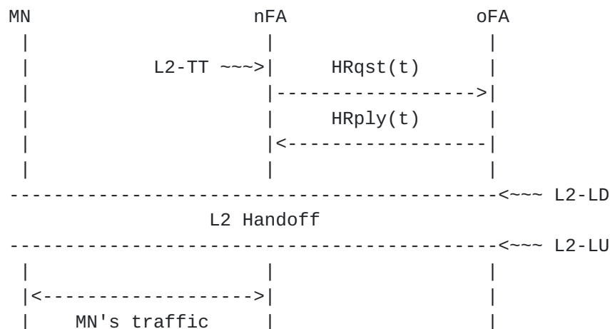
Figure 8 - Two Party Target Trigger Handoff Timing
