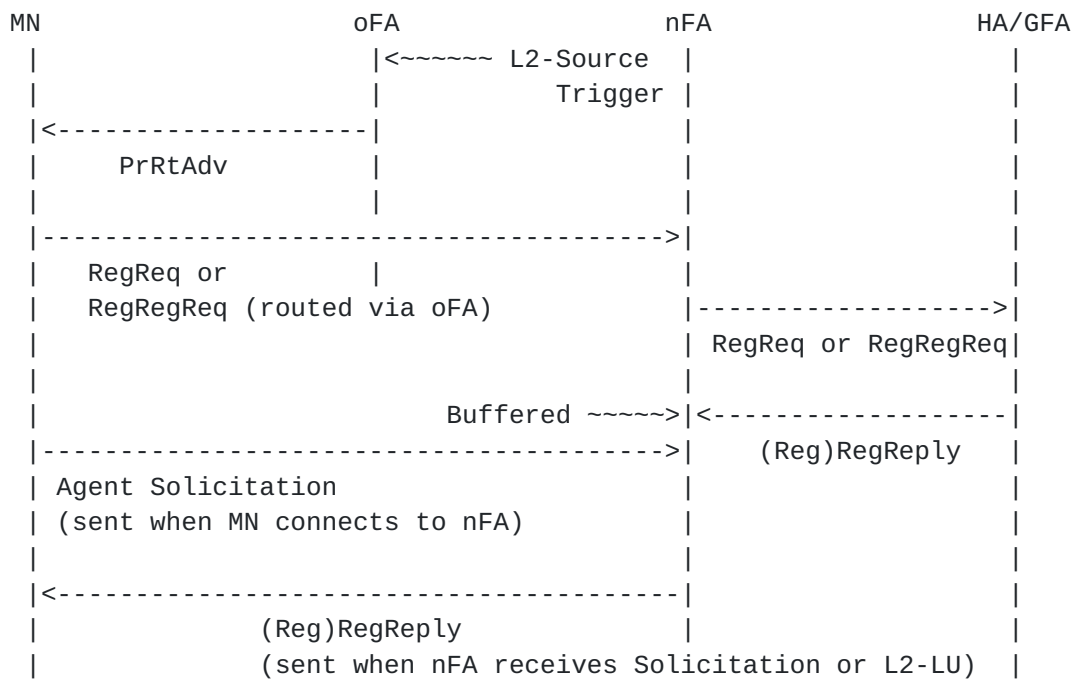
Figure 2 - PRE-REGISTRATION Handoff Message Timing Diagram
