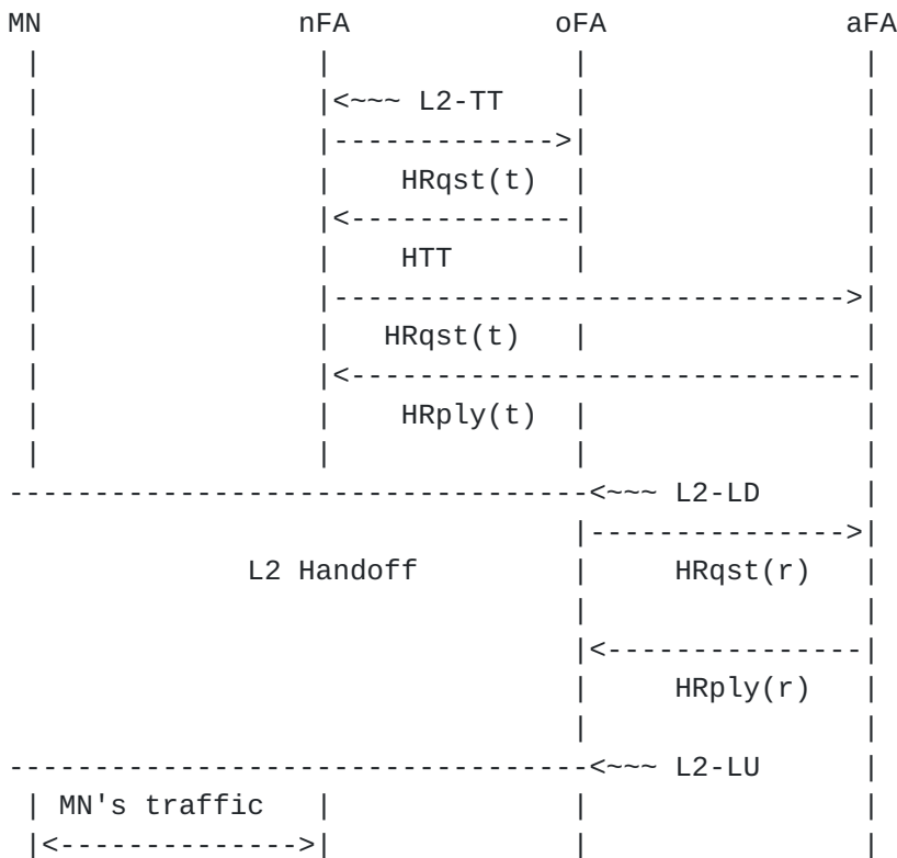
Figure 11 - Three Party Target Trigger Handoff Timing
