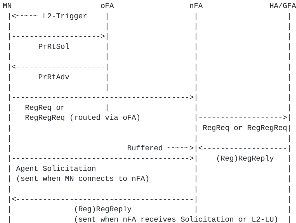
Figure 4 - PRE-REGISTRATION Handoff Message Timing Diagram (Mobile-Initiated)
