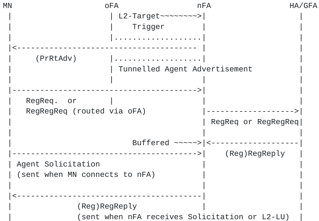
Figure 3 - PRE-REGISTRATION Handoff Message Timing Diagram (Network-Initiated, Target Trigger)
