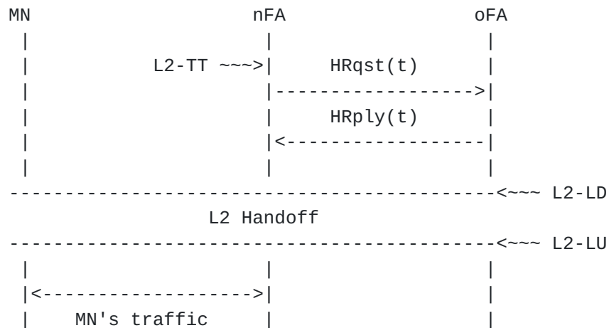
Figure 8 - Two Party Target Trigger Handoff Timing
