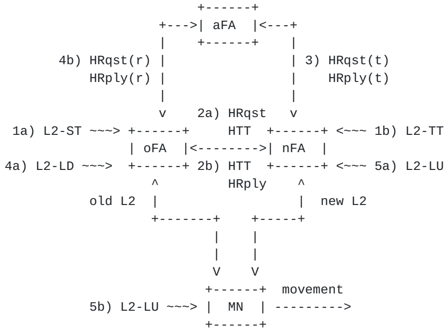
Figure 9 - Three Party Handoff
