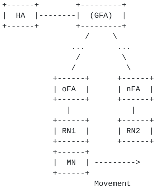
Figure B.1 - Network Model for Mobile IPv4 With Multi-Access
