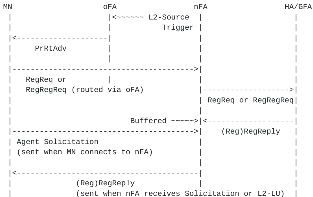
Figure 2 - PRE-REGISTRATION Handoff Message Timing Diagram
