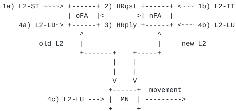
Figure 6 - Two Party Handoff (POST-REGISTRATION)
