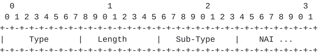
Figure 4: The Generalized NAI (GNAI) Extension
