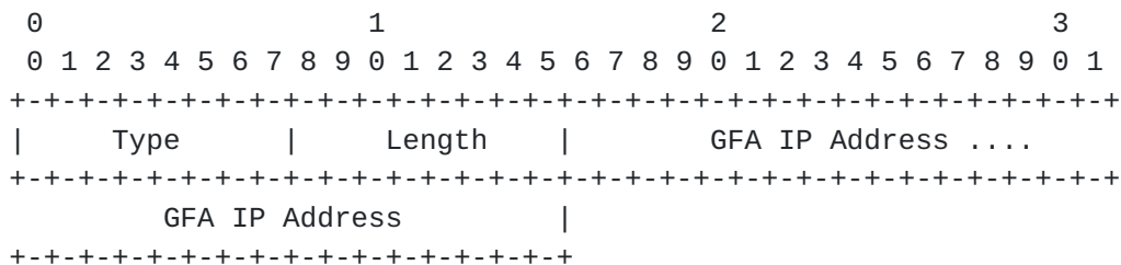
Figure 5: The GFA IP Address extension
