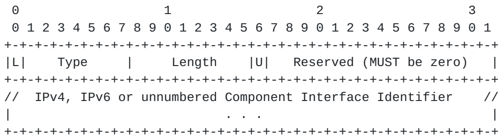
Figure 1: Component Interface Identifier ERO subobject
