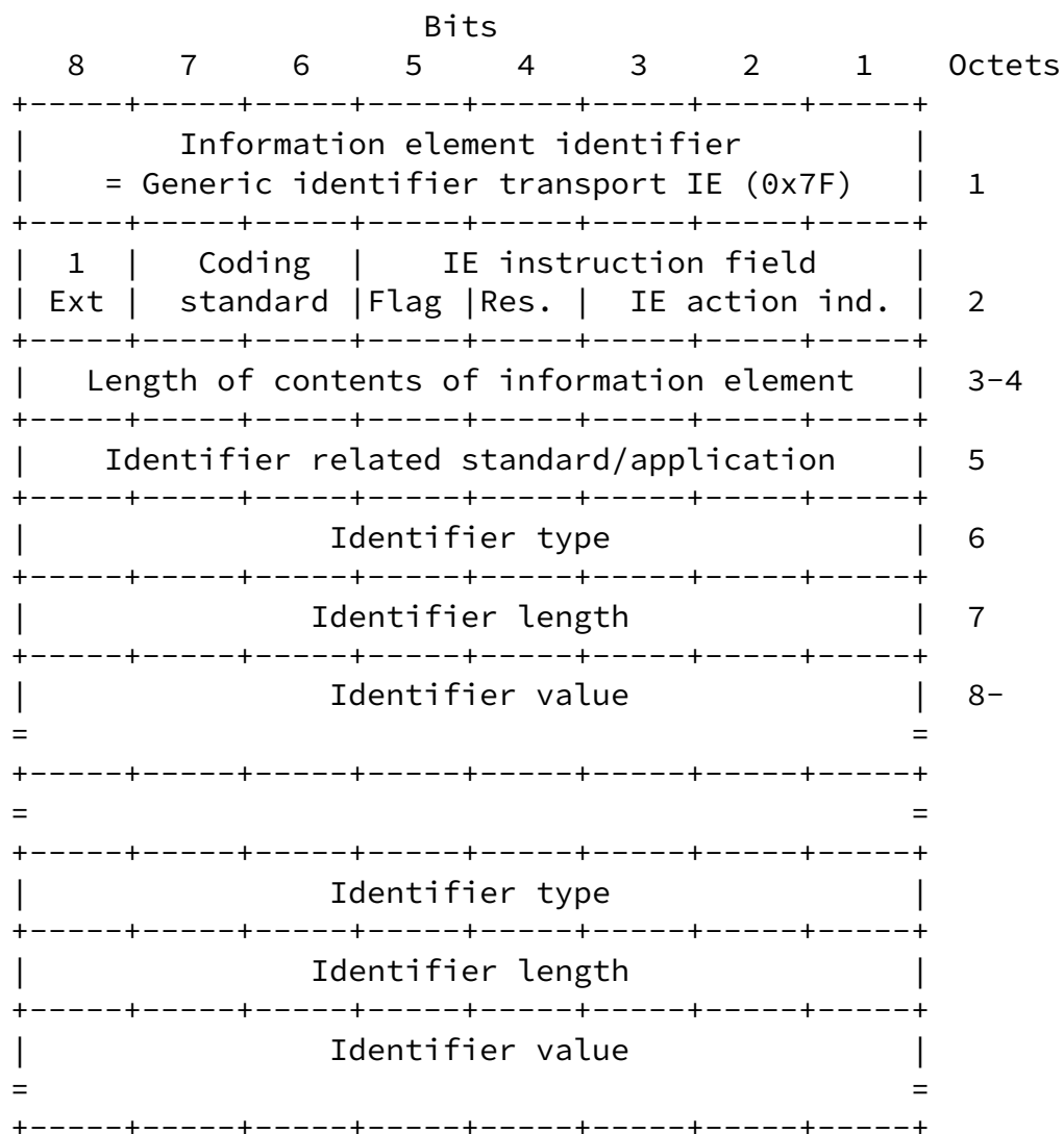
Fig. 3.1: Format of the Generic Identifier information element.
