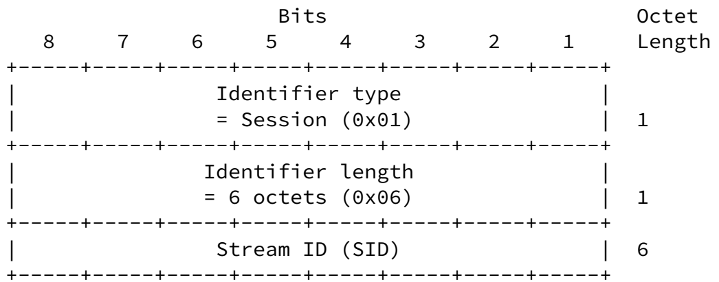
Fig. 4.3: ST2+ session identifier.
