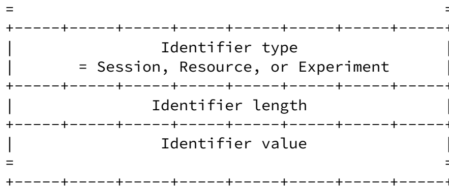
Fig. 4.1: Principle of assignment in the Generic Identifier information element.
