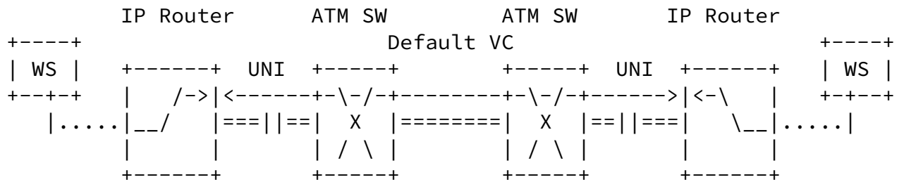
A. New session initially forwarded over a default VC.
