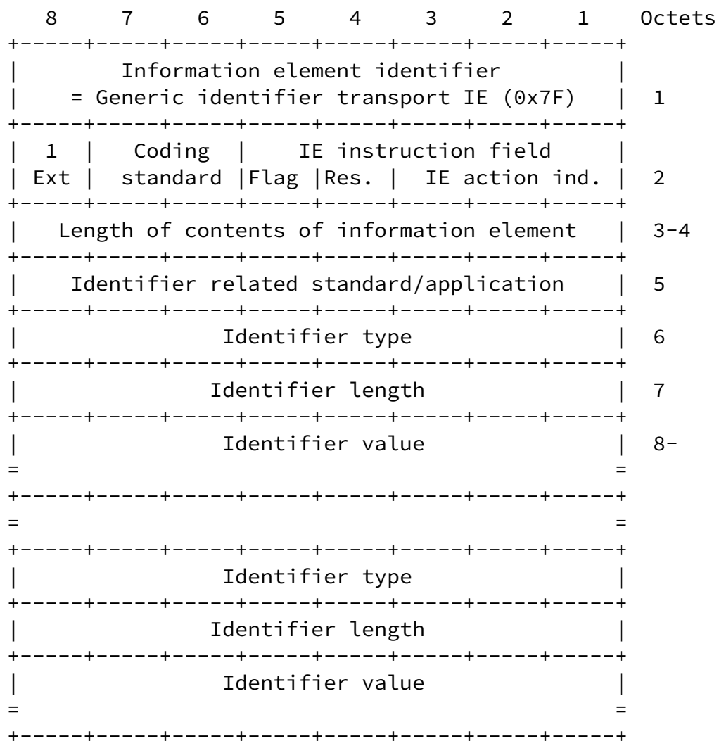
Fig. 3.1: Format of the Generic Identifier information element.
