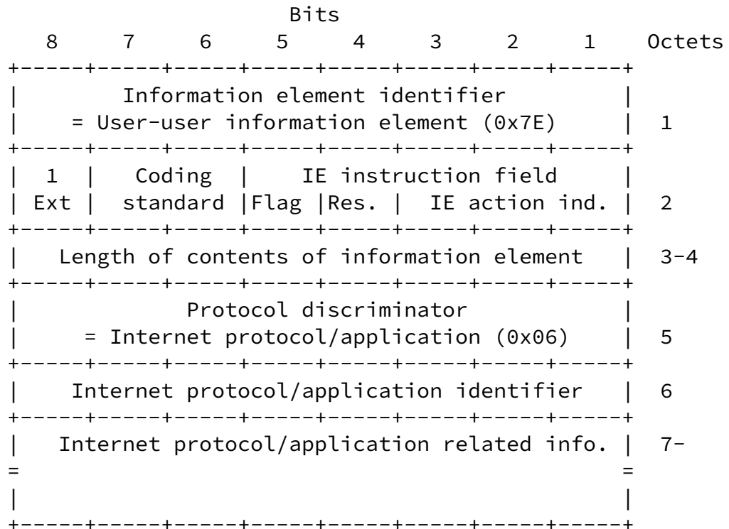
Fig. 4.7: Principle of assignment in the User-user information element.
