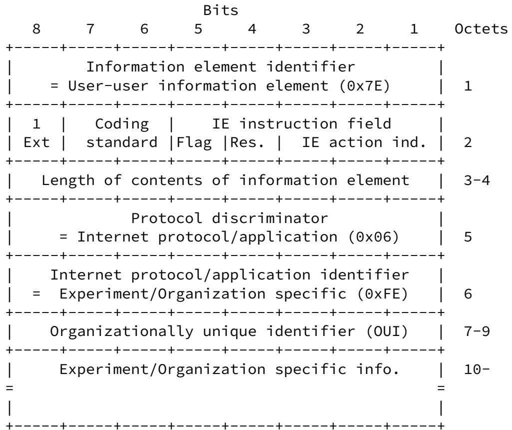
Fig. 4.10: Experiment/Organization specific.
