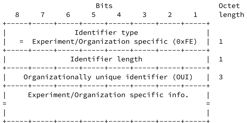
Fig. 4.6: Experiment/Organization specific.
