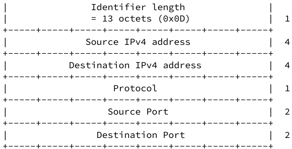
Fig. 4.2: IPv4 session identifier.
