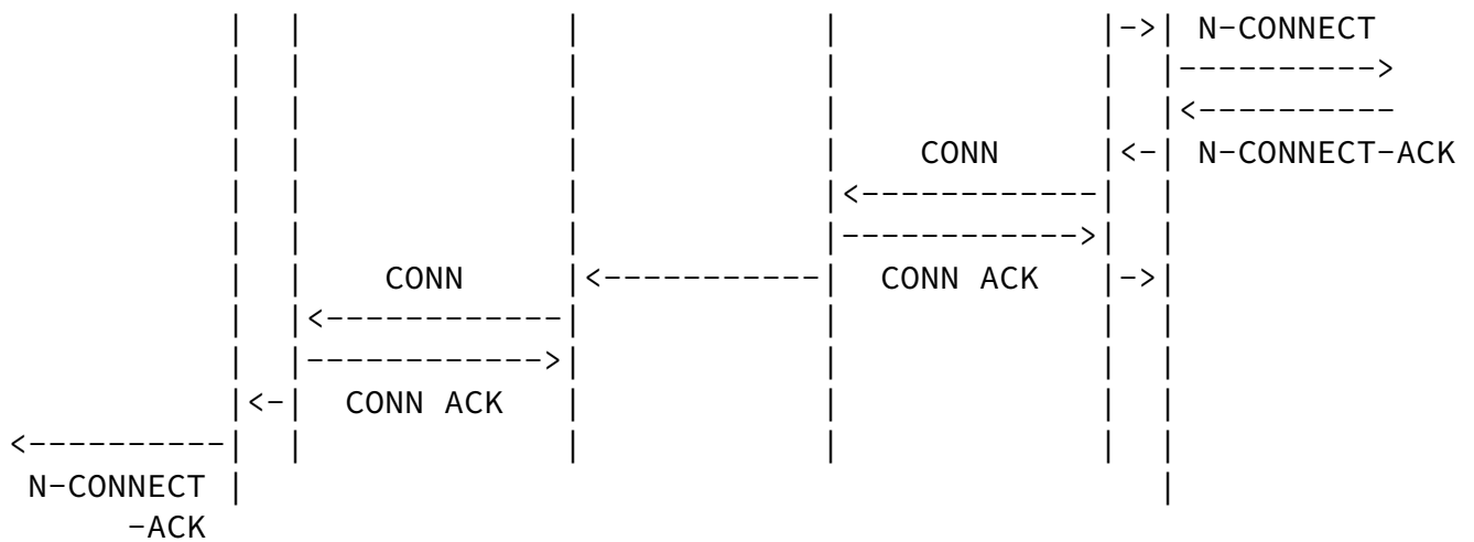
Fig. 2.2: Example procedure for simultaneous QoS-sensitive session and ATM VC establishment.
