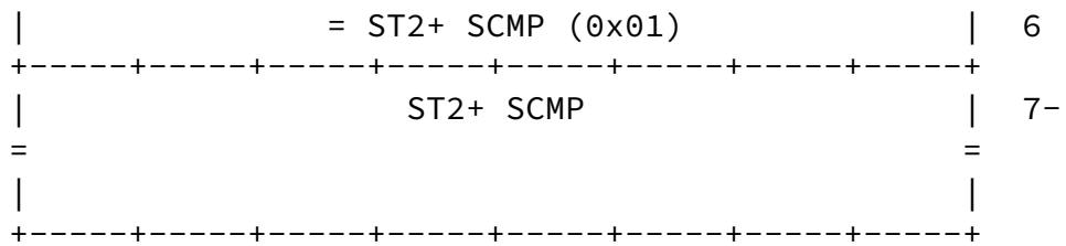
Fig. 4.8: ST2+ SCMP.
