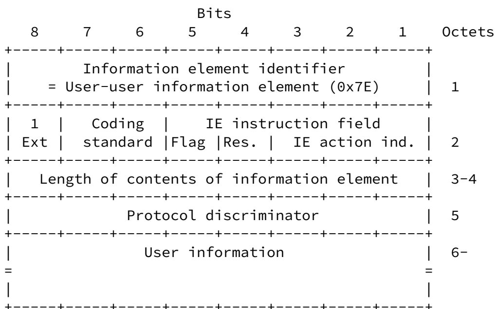
Fig. 3.2: Format of the User-user information element.
