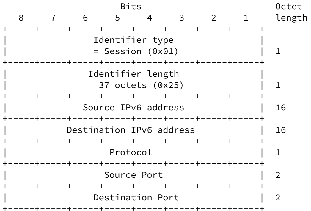
Fig. 4.4: IPv6 session identifier.
