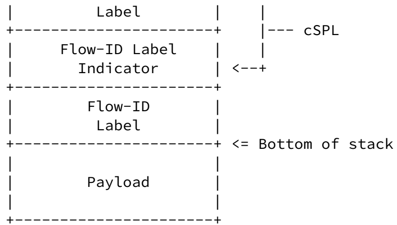
Figure 3: Applying Flow-ID to MPLS VPN
