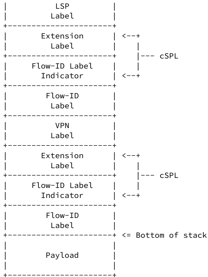
Figure 4: Applying Flow-ID to both MPLS LSP and MPLS VPN
