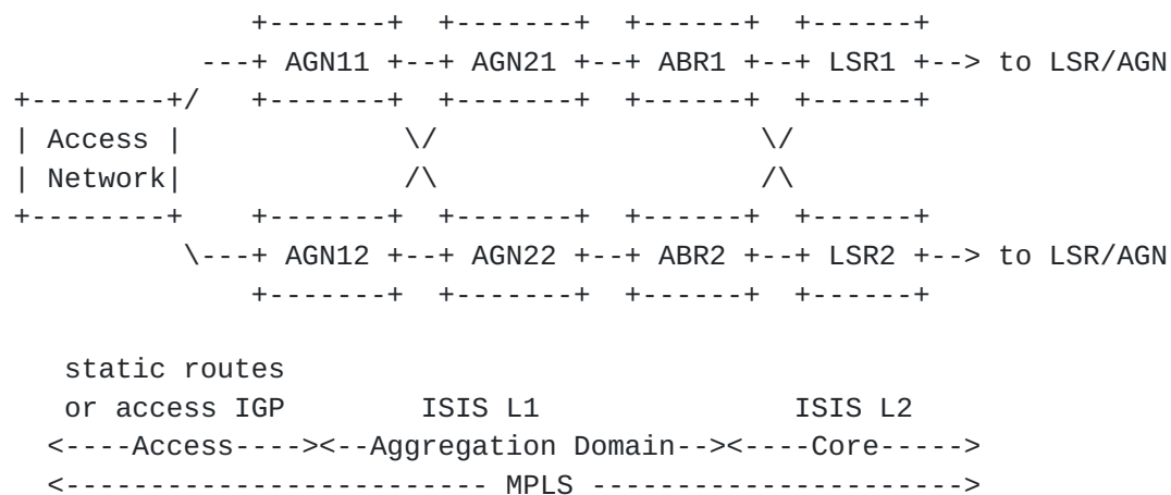
Figure 1: Seamless MPLS end-to-end reference network topology.
