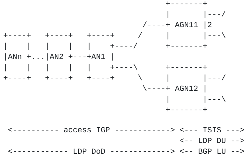
Figure 6: [Y] access topology with access IGP.
