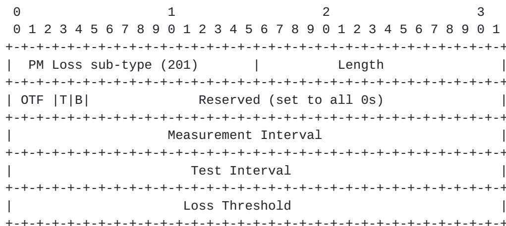
Figure 8: PM Loss Measurement sub-TLV format
