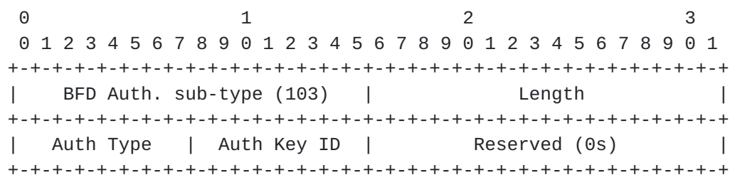
Figure 5: BFD Authentication sub-TLV format
