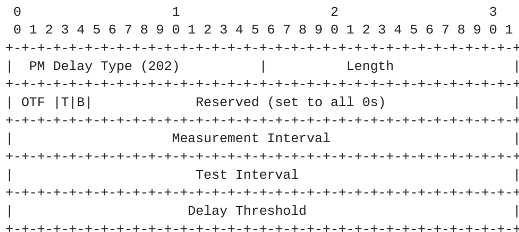
Figure 9: PM Delay Measurement sub-TLV format
