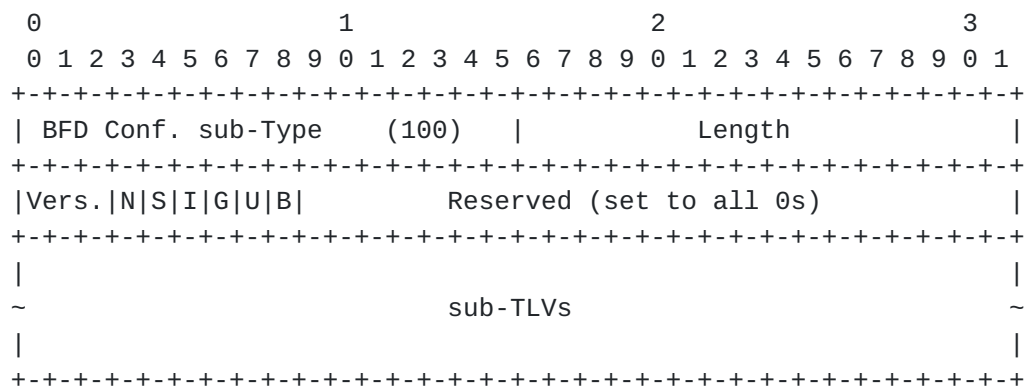
Figure 2: BFD Configuration sub-TLV format
