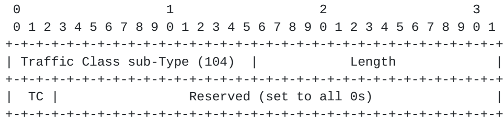
Figure 6: Traffic Class sub-TLV format
