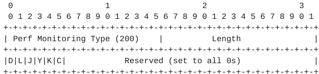
Figure 7: Performance Measurement sub-TLV format
