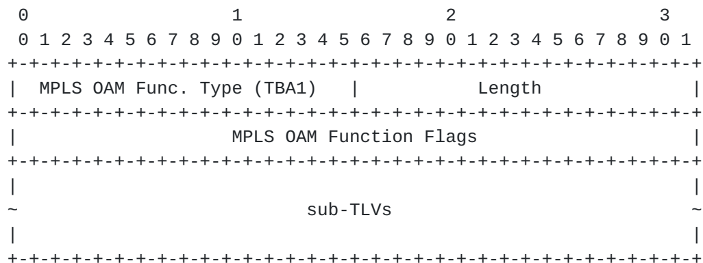
Figure 1: MPLS OAM Functions TLV format
