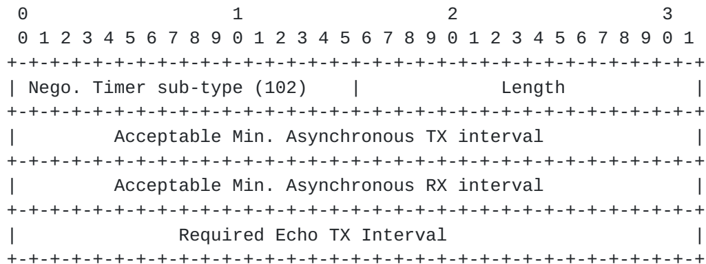
Figure 5: Negotiation Timer Parameters sub-TLV format
