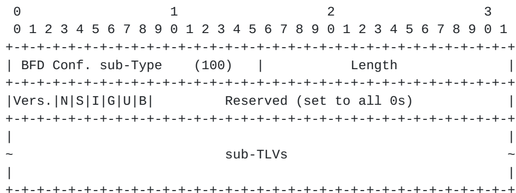
Figure 3: BFD Configuration sub-TLV format
