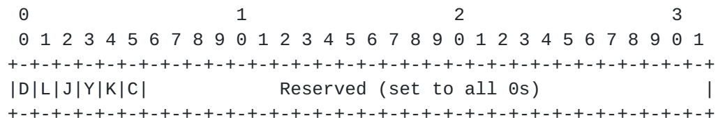
Figure 9: Performance Measurement sub-TLV format
