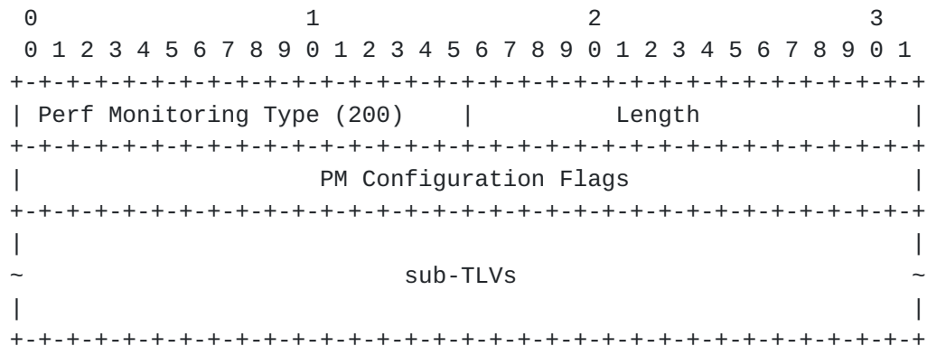
Figure 8: Performance Measurement sub-TLV format
