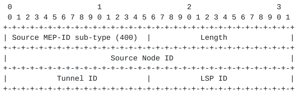
Figure 13: Source MEP-ID sub-TLV format
