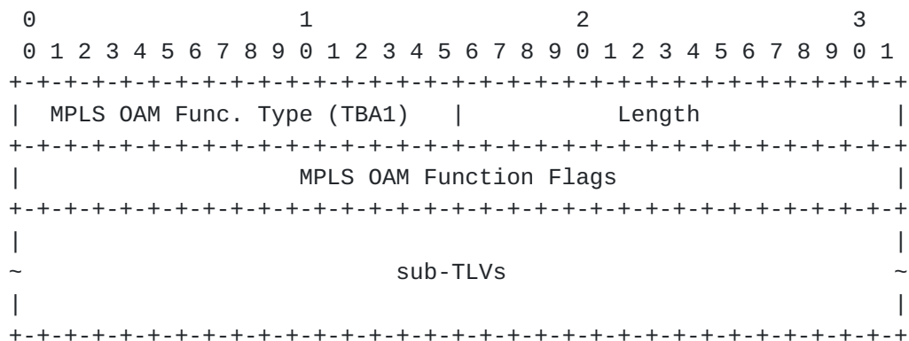
Figure 1: MPLS OAM Functions TLV format
