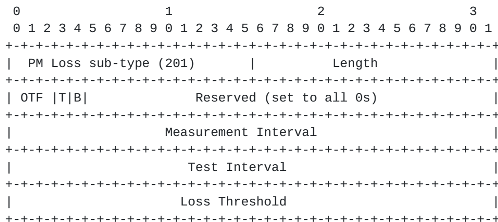
Figure 10: PM Loss Measurement sub-TLV format
