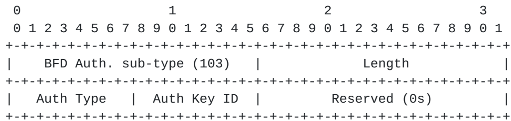
Figure 6: BFD Authentication sub-TLV format
