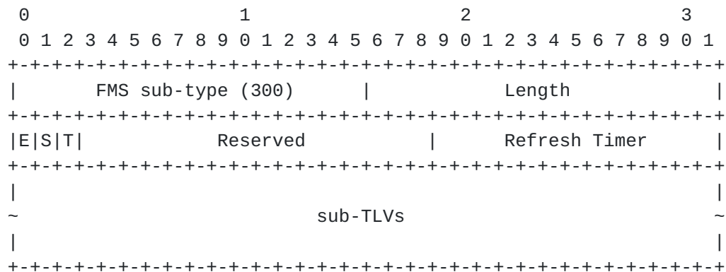
Figure 12: Fault Management Signal sub-TLV format
