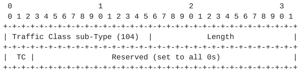
Figure 7: Traffic Class sub-TLV format
