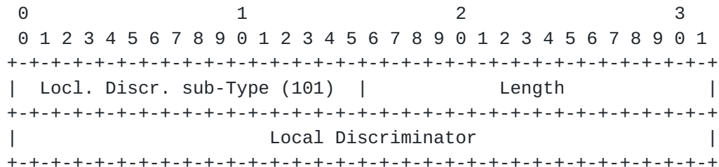
Figure 4: Local Discriminator sub-TLV format
