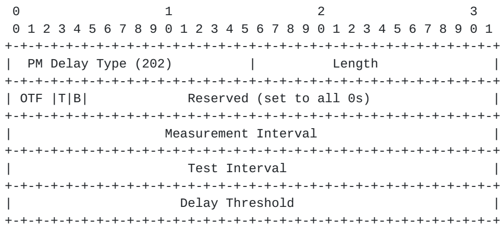
Figure 11: PM Delay Measurement sub-TLV format
