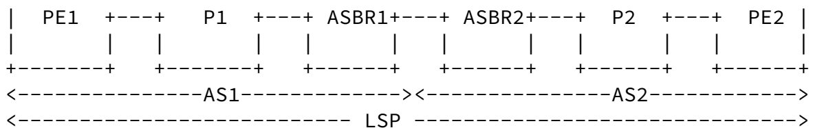
Figure 4: Example Inter-AS LSP
