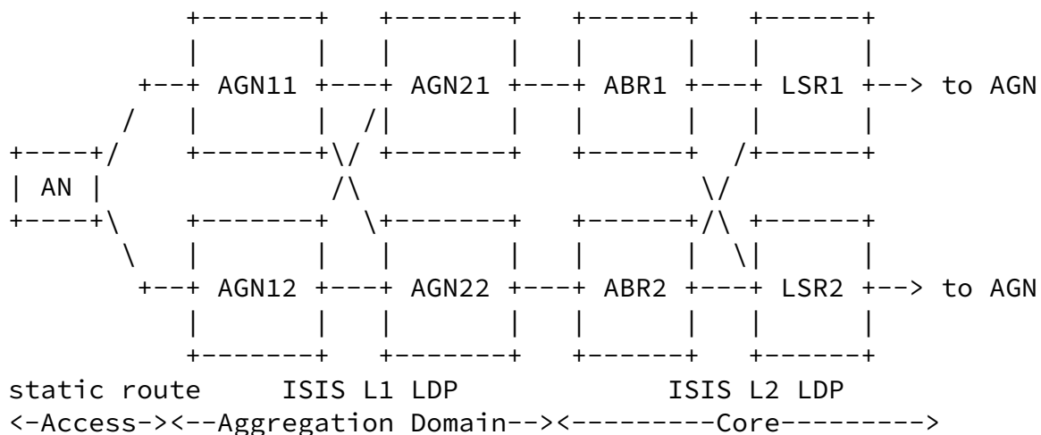
Figure 2: Seamless MPLS Architecture
