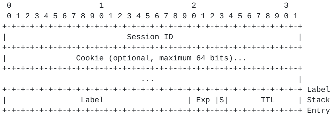
Figure 2.2 MPLS over L2TPv3 encapsulation
