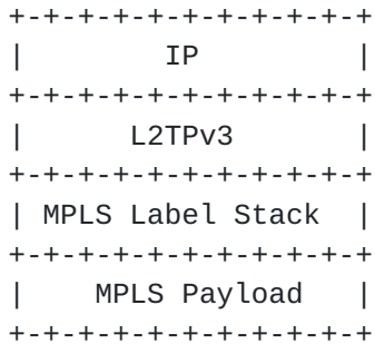
Figure 2.1 MPLS Packet over L2TPv3/IP
