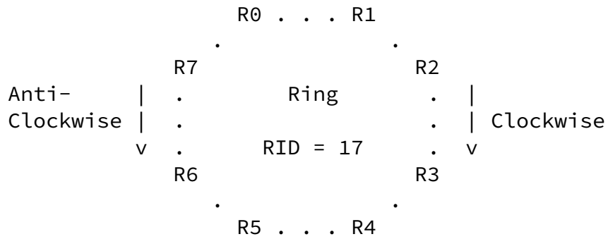
Figure 1: Ring with 8 nodes
