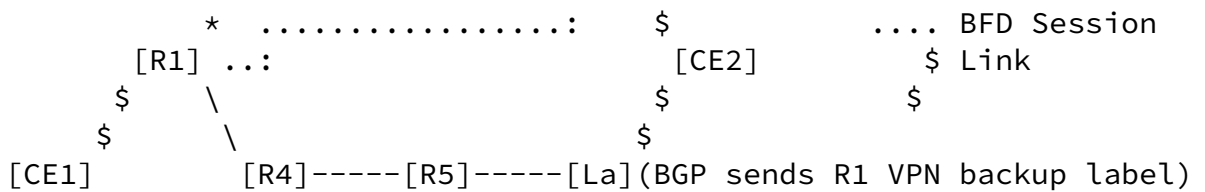
Figure 2: Protect Egress for L3VPN Traffic
