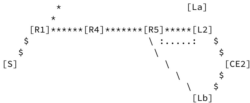
Figure 1: Backup LSP for Locally Protecting Egress
