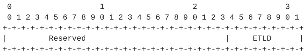
Figure 8: The ETLD Attributes TLV
