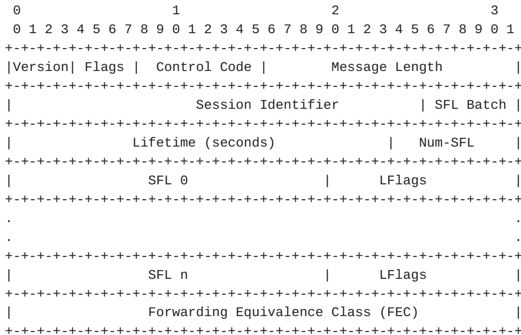
Figure 1: SFL Control Message Format
