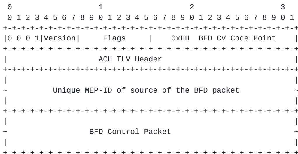
Figure 3: MPLS CV Message
