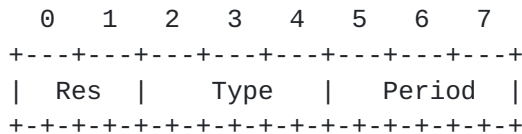
Figure 3 Format of Flags in CSF PDU
