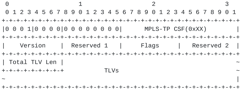
Figure 2 Frame format of CSF
